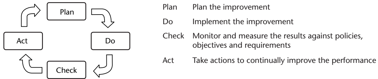
Figure 2-1. PDCA cycle
