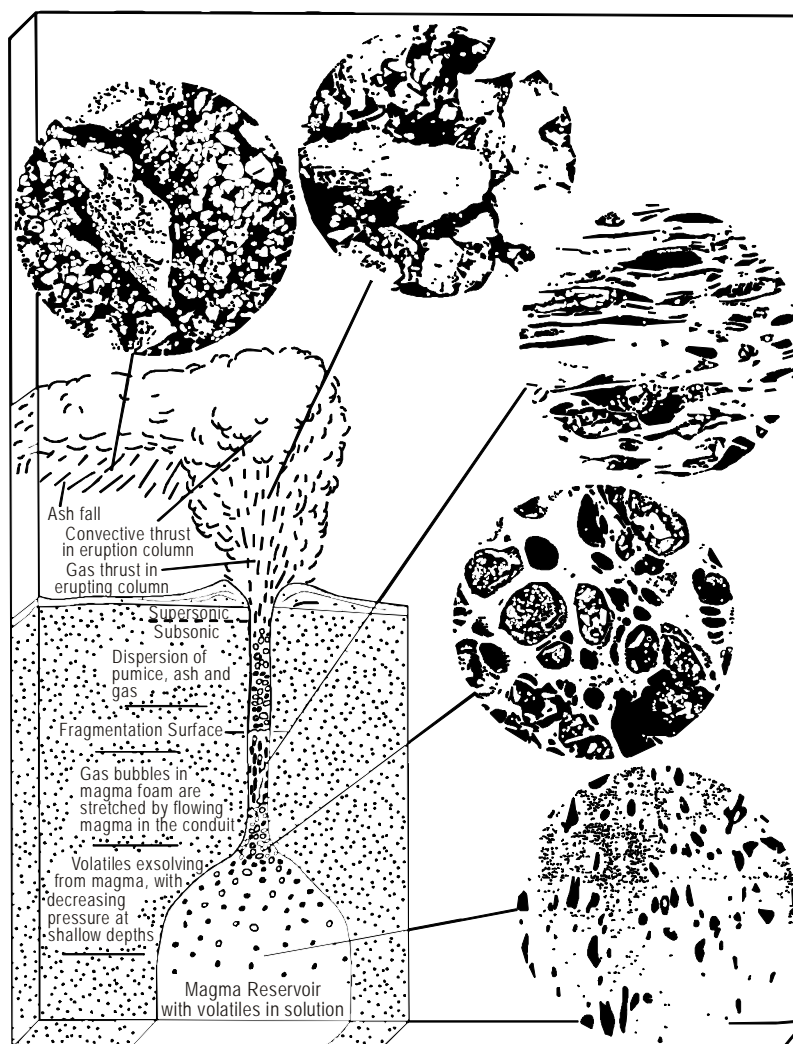
Figure 1-2. Schematic diagram of processes leading to the formation of volcanic ash within explosive volcanic eruptions. This diagram is based nearly entirely on inference and some experimental studies of the processes of gas exsolution and explosive decompression of a rising magma with a composition similar to that found in the eruptions of Augustine Volcano. Scanning electron photomicrographs shown in the circles are about 300 \mu\text{m} ( 300 \times 10^{-6} metres) in diameter. As magma rises to a depth where the pressure of gas in solution exceeds that of the overlying rock, some of that gas comes out of solution as small bubbles. As the pressure is lowered, those bubbles continue to grow. After the eruption begins, movement of the magma foam in the conduit may stretch the bubbles into elongate, tapered tubes. A fragmentation surface between the pressurized magma foam and the ambient atmosphere tears the brittle foam apart and accelerates the pieces out of the conduit in the eruption column. The particles are carried into eruption clouds and eventually fall to the ground, their final position depending on the height of the eruption column, the strength of winds, and particle size and density. (The samples used here to demonstrate the appearance of volcanic ashes, within the eruption column are from coarse ash fallout deposits — in situ samples from eruption columns have never been collected.) (from Heiken)
