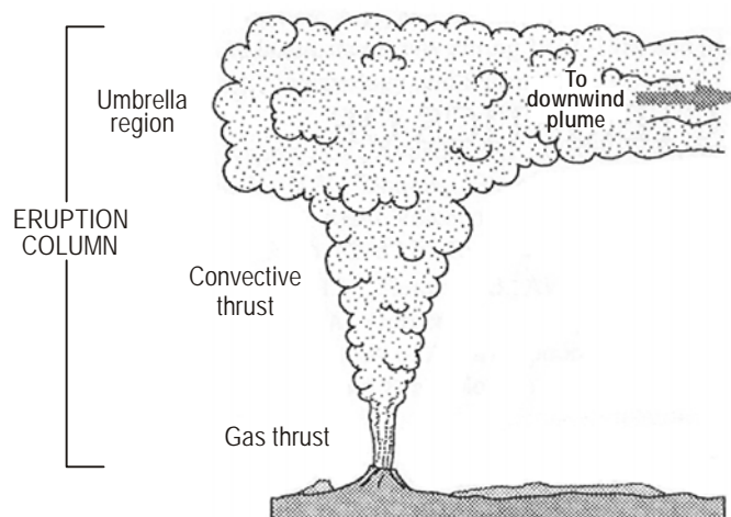
Figure 2-4. Three parts or regions of an eruption column: gas thrust, convective thrust and umbrella. (from Self and Walker)
