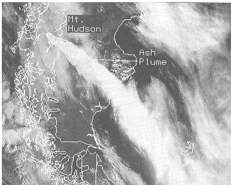
Figure 3-4. Infrared image from the NOAA 10 polar-orbiting weather satellite on 15 August 1991 at about 0800, showing ash column extending SE from Hudson. Temperature estimates suggest that the column is at about 17-18 km altitude. (courtesy of Synoptic Analysis Branch, NOAA/NESDIS, from Global Volcanism Network)
