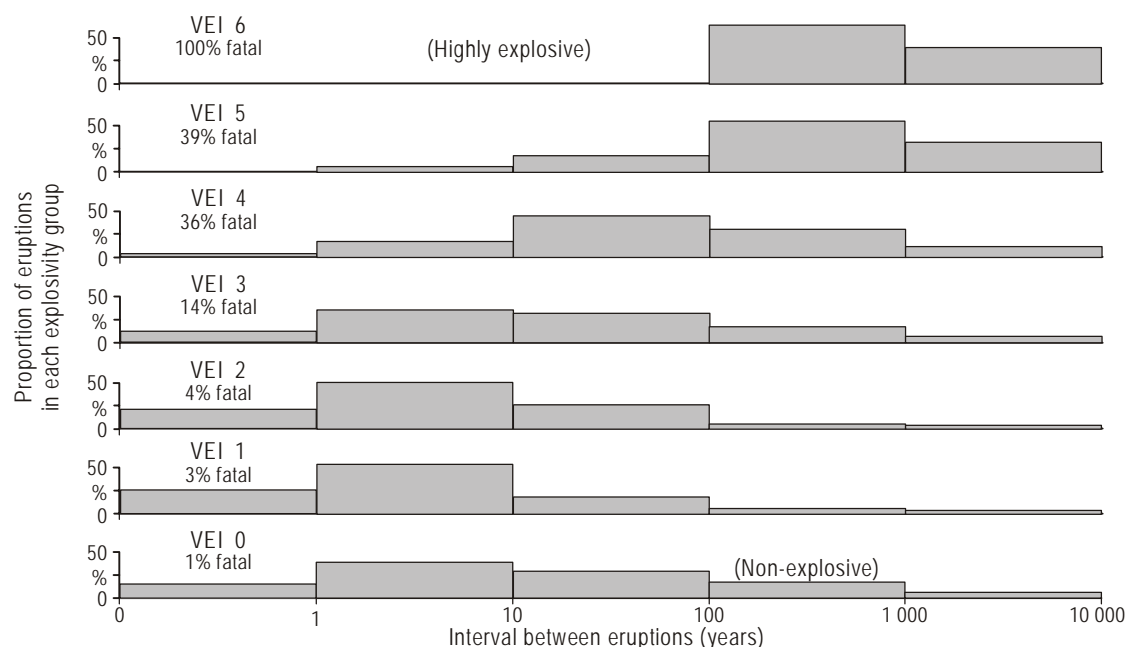
Figure 1-3. Explosivity and time intervals between eruptions. For each VEI unit, eruptions are grouped by time interval from start of previous eruption. The number of eruptions in VEI groups 0 to 6 are, respectively: 446, 677, 2 991, 692, 230, 48 and 16. For each group, the percentage of historical eruptions that have been fatal is also shown to emphasize the danger of large explosive eruptions from volcanoes that have appeared to be quiet for hundreds to thousands of years. (from Simkin and Siebert)
