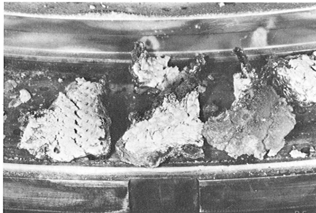
Figure 4-1 b). Leading-edge deposits dislodged during disassembly of stage-1 high-pressure-turbine nozzle guide vanes. (from Przedpelski and Casadevall)
