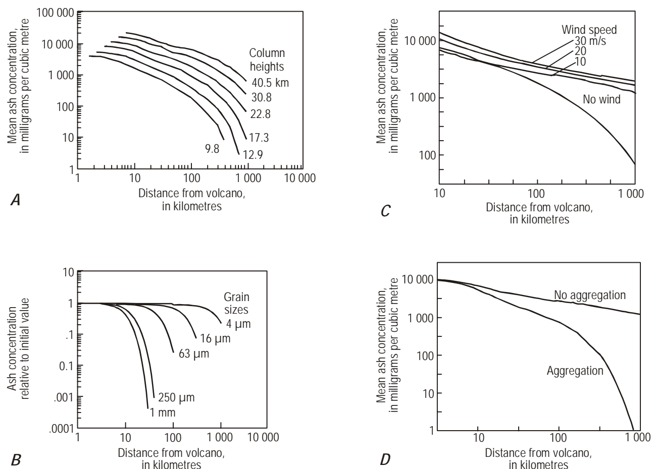
Figure 2-7 A. Ash concentration in an umbrella cloud (in \text{mg}/\text{m}^3 ) is plotted against distance for six different column heights and for dispersal in the absence of wind.
