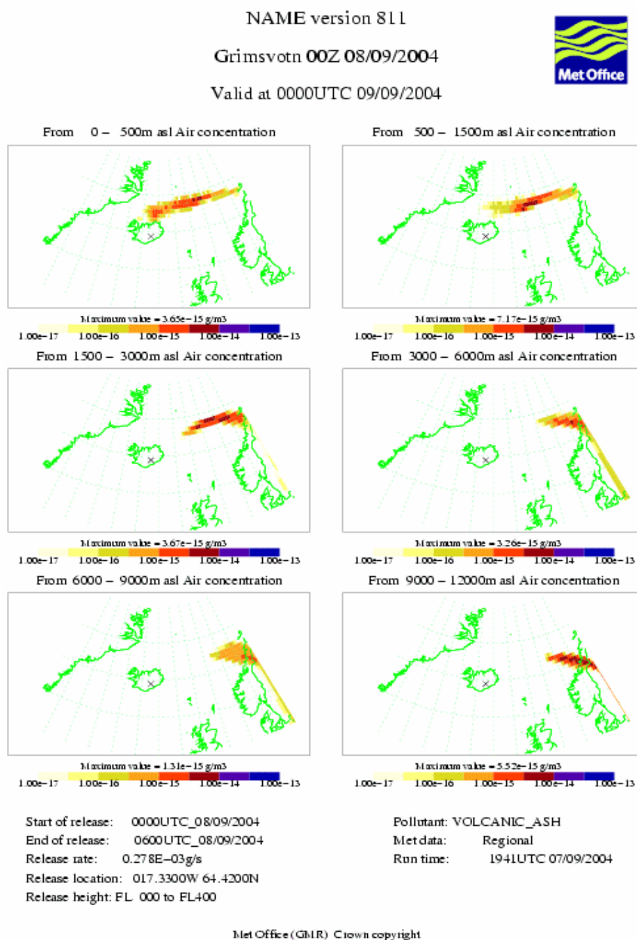
Figure 3-8. NAME forecasted dispersion for a hypothetical eruption of Mt. Grimsvötn.
