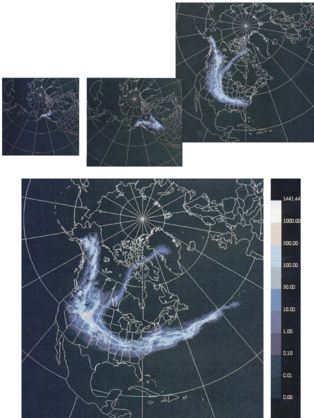
Figure 3-7. Mt. Redoubt erupts. In this example of an output from the tracer model developed by the Atmospheric Environment Service of Canada, the four panels depict the simulated dispersion of volcanic ash cloud after the eruption of Mt. Redoubt at 1900 hours UTC on 14 December 1989. The concentrations are indicated in a logarithmic scale. The panels refer to the 250 hPa level and correspond to the situation at 12 hours, 24 hours, 36 hours and 48 hours after the eruption. (from ICAO Journal)
