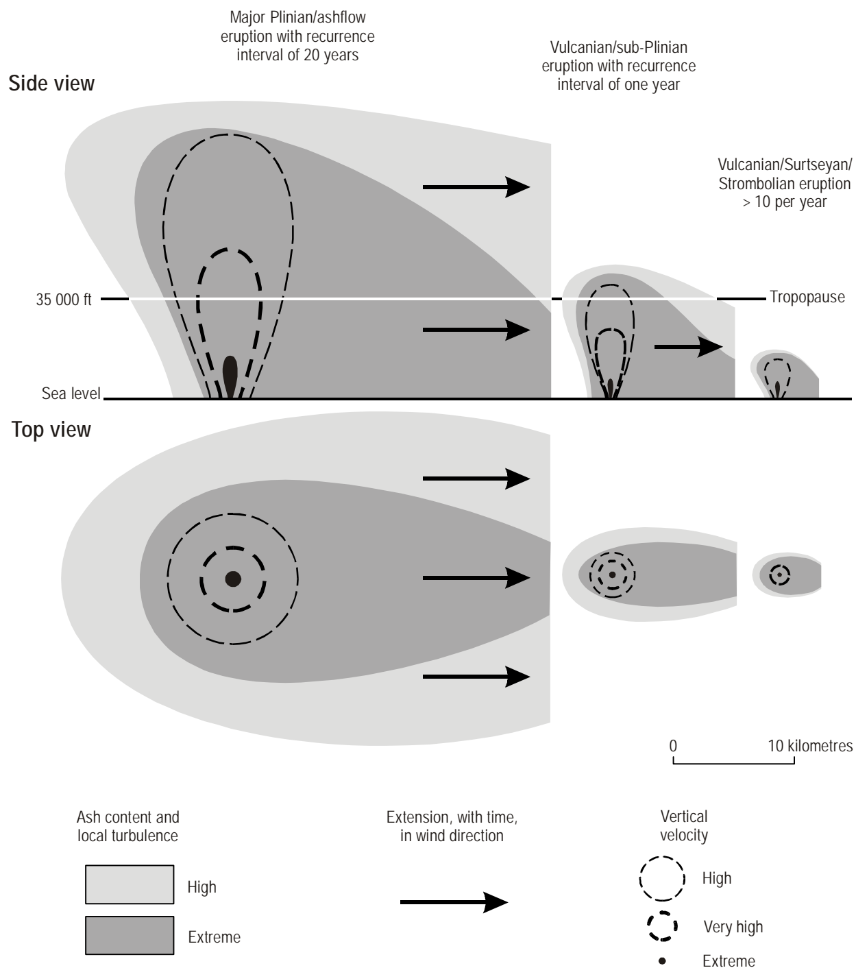
Figure 1-4. Schematic diagram showing the distribution of hazards to aircraft around explosive eruption columns of three selected frequencies.
