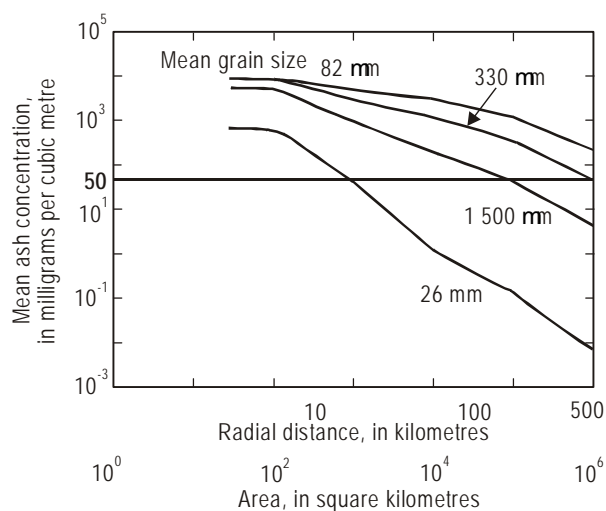
Figure 2-2. Concentration variation for different total grain-size distributions with means shown next to curves. The standard deviation, in \sigma units, for each curve was assumed to be 2.5. Distributions are for phreato-Plinian/coignimbrite (mean = 82 \mu m), Vulcanian (330 \mu m) and Strombolian (26 \mu m) eruptions. (from Woods and Bursik).
