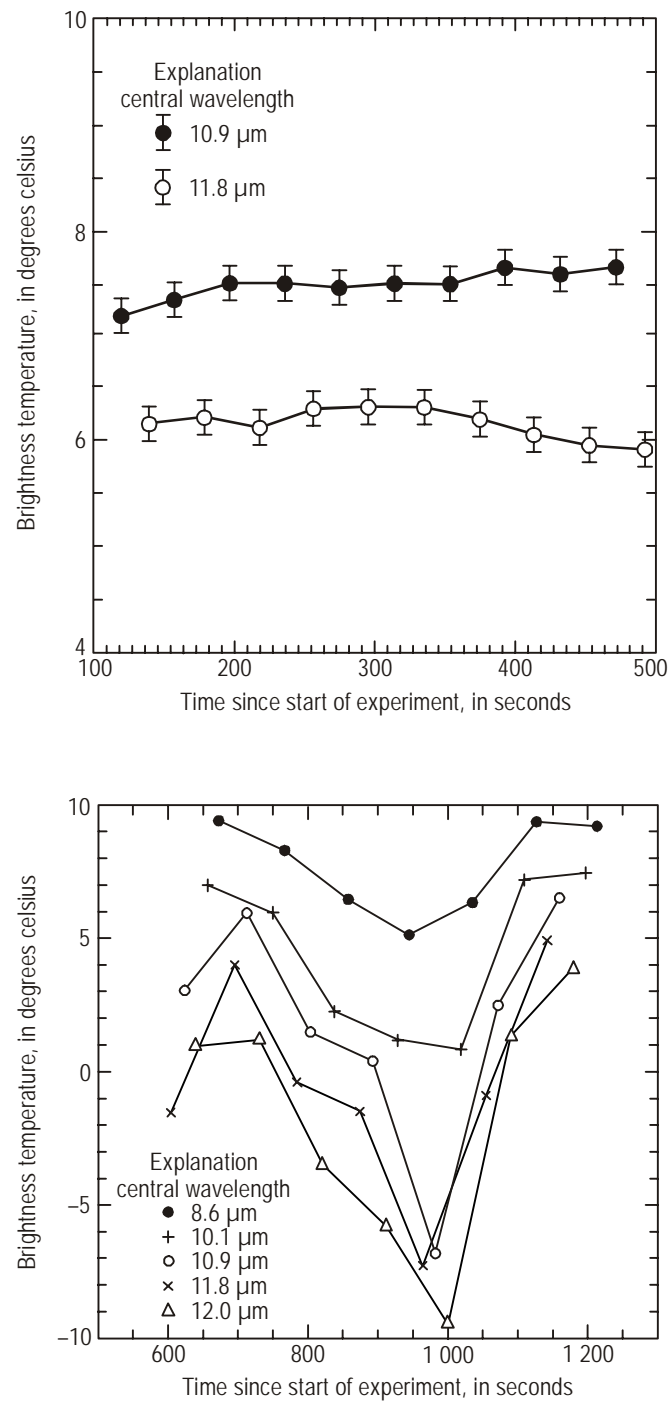
Figure 3-6. (Top) Ground-based measurements of a cumulus cloud near Mt. Sakurajima, Japan, 10 March 1991, radiometer looking at an elevation of 21°. Vertical bars indicate measurement uncertainty. (Bottom) Ground-based measurements of volcanic ash cloud emanating from Mt. Sakurajima, Japan, 10 March 1991. Radiometer looking at an elevation of 13.5°. (from Prata and Barton)
