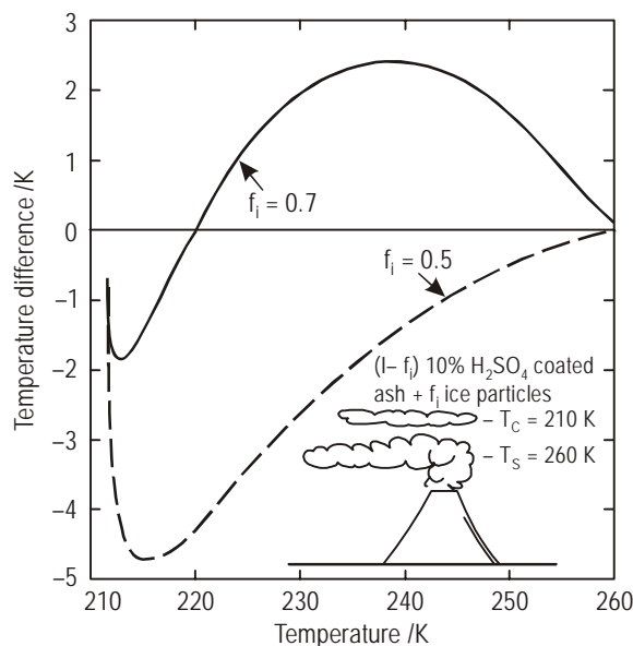
Figure 3-1. Temperature difference ( T_4 - T_5 ) as a function of T_4 temperature for a mixture of ash and ice particles. (from Prata)
