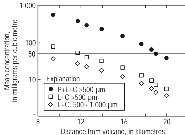
Figure 2-6. Inferred concentration of pyroclasts in the Fogo umbrella cloud as a function of distance from the vent along the dispersal axis. Concentrations in other directions would be somewhat lower. P, pumice; L, lithic (rock) fragments; C, crystals. (from Bursik, Sparks, Carey and Gilbert).
