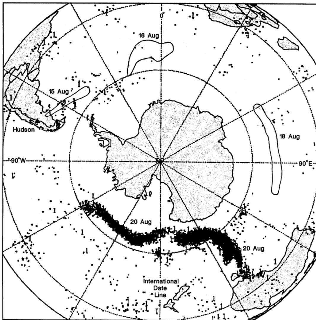
Figure 3-5. Polar view of SO 2 column from Hudson: preliminary data from the total ozone mapping spectrometer (TOMS) on the Nimbus-7 satellite showing an eruption cloud from Hudson on 20 August 1991 at about 1100 (local time). Each dot represents SO 2 values about 10 milliatmosphere-cm (100 ppm-m), within an area 50 km across. The prominent concentration of SO 2 to the left represents the cloud's position 24 hours after that to the right, but both are 20 August because they straddle the International Date Line. Envelopes surrounding the cloud's position at approximately 1100 (local time) on 15, 16 and 18 August have been added to illustrate its passage around the globe. (courtesy of Scott Doiron from Global Volcanism Network)
