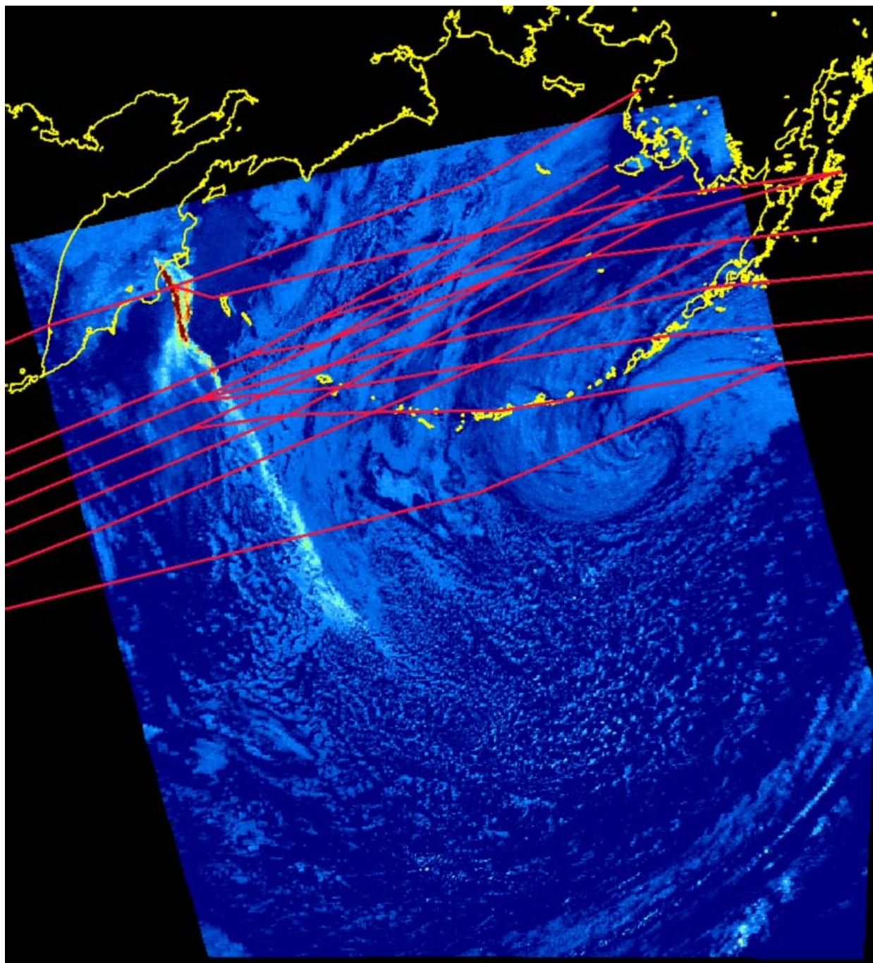
Figure 3-2 a). AVHRR split-window image of the volcanic ash cloud from Klyuchevskoi Volcano, collected on 1 October 1994 at 0640Z. Both the proximal and distal regions of the ash cloud are highlighted using this method. (courtesy of D. Schneider, U.S. Geological Survey, Alaska Volcano Observatory.)
