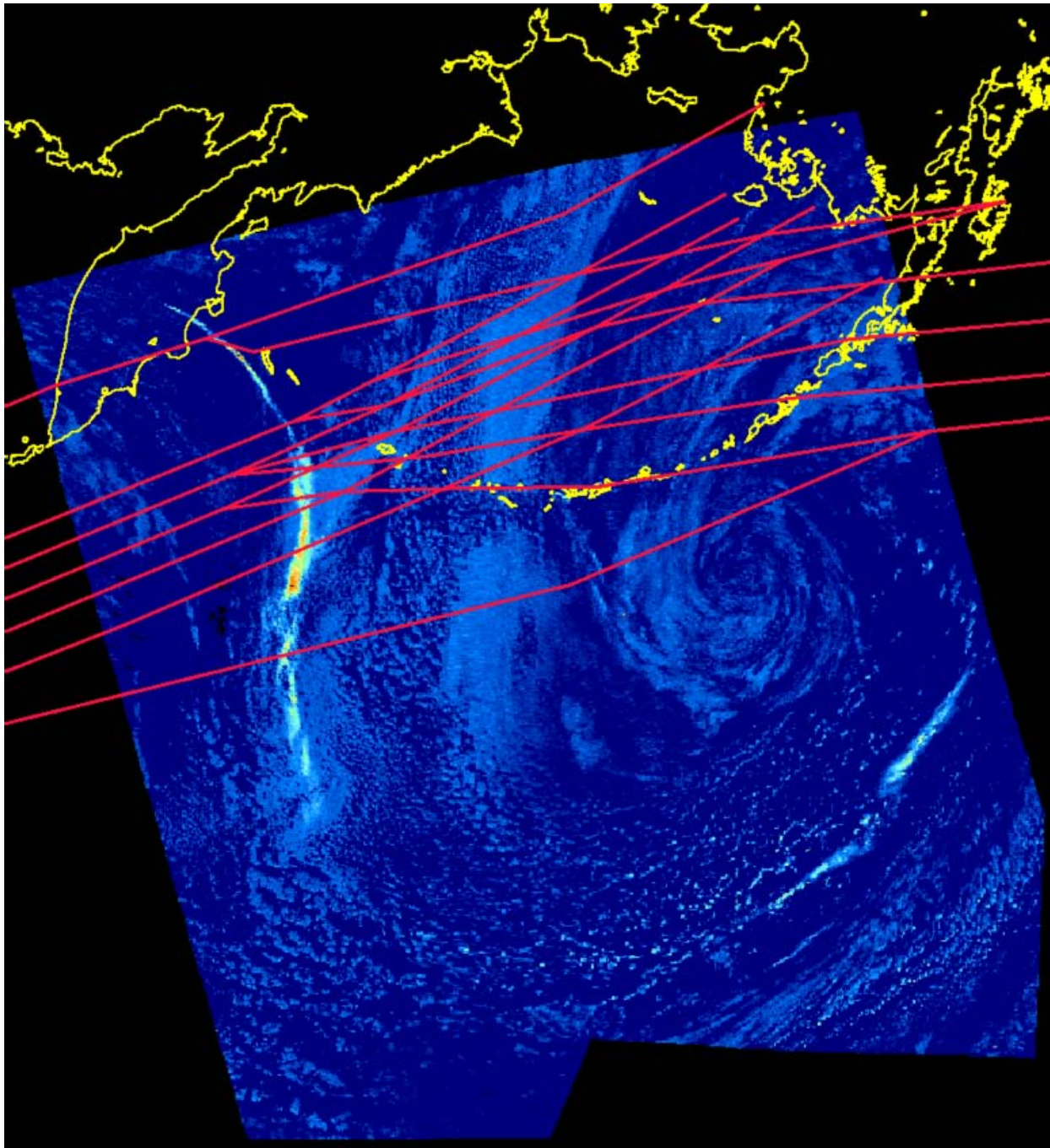
Figure 3-2 b). A composite AVHRR split-window image of the volcanic ash cloud from Klyuchevskoi Volcano, collected on 1 October 1994 at 1900Z and 2030Z. The distal ash cloud is observed crossing many of the North Pacific air routes in this image. The extent of this cloud was difficult to discern without using this method. (courtesy of D. Schneider, U.S. Geological Survey, Alaska Volcano Observatory.)
