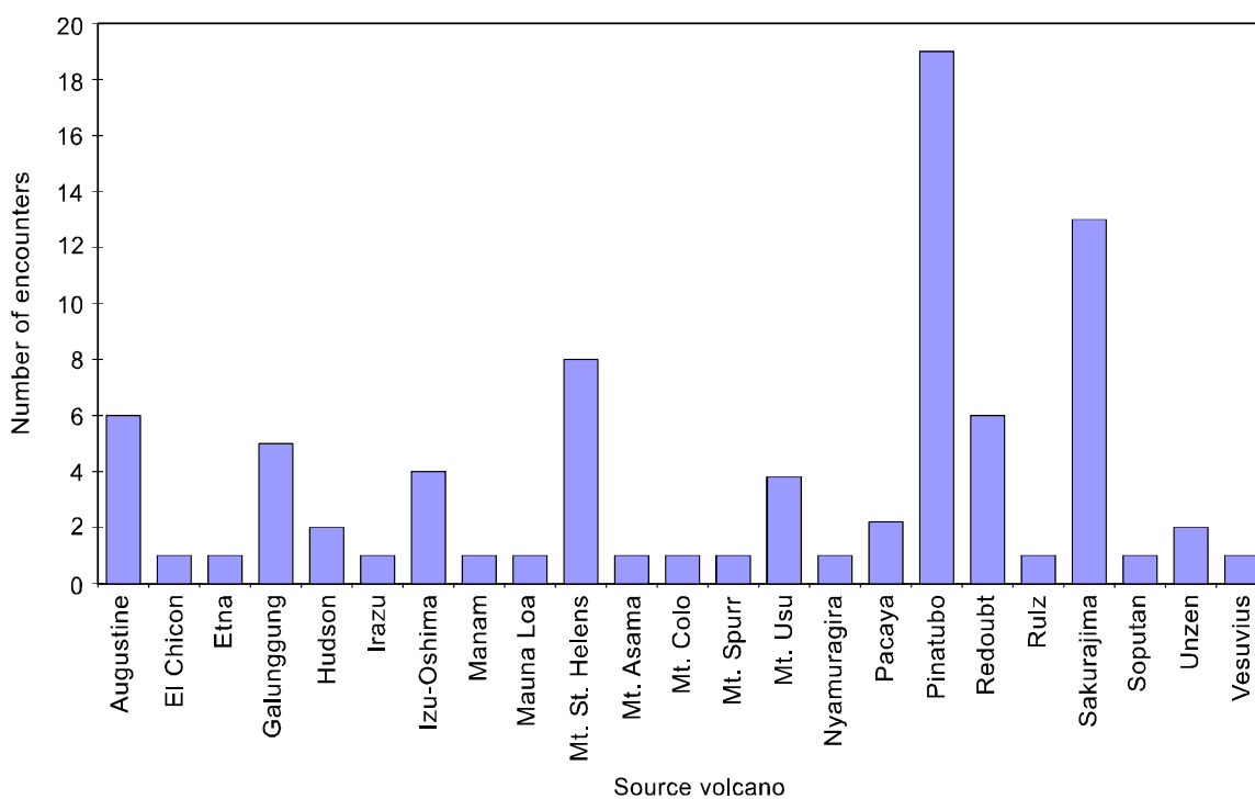
Figure 3. Plot showing the number of aircraft/volcanic ash encounters relative to the source volcano producing the eruption
