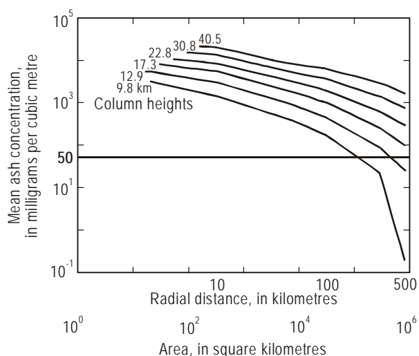
Figure 2-3. Ash concentration as a function of the area encompassed by an isochronous surface within the umbrella cloud for column heights from 10 to 40 km (30 000 to 45 000 ft). (Isochronous meaning measured at the same time.) (from Woods and Bursik)
