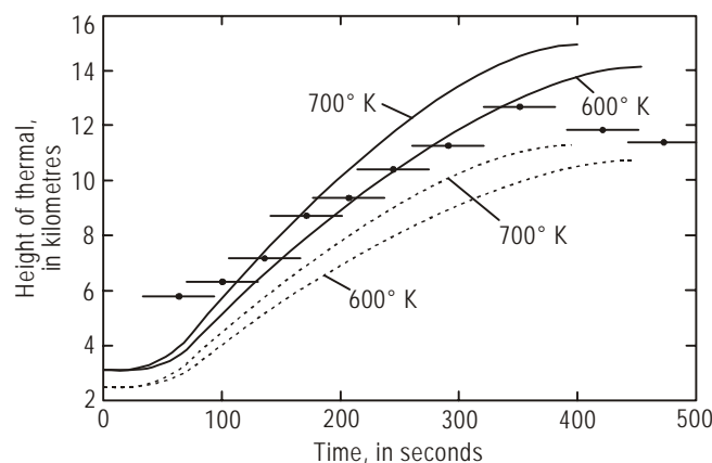
Figure 2-5. Comparison of observed ascent of the 15 April 1990 Redoubt eruption cloud with the model predictions of the total cloud height (solid lines) and the height of the centre of the cloud (dashed lines). Calculations are shown for two initial model cloud temperatures (600°K and 700°K), which represent bounds on the initial temperature of the cloud (from Woods and Kienle). The data were collected by analysis of video recordings of the cloud ascent. Horizontal lines through data points represent error bars.
