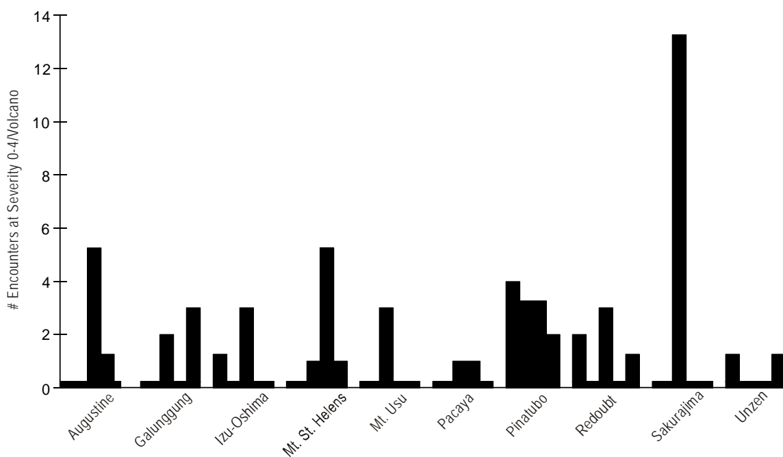
Figure 4. Plot showing the number of aircraft/volcanic ash encounters for each class (from 0 to 4) of encounter severities that occurred at the given source volcano
