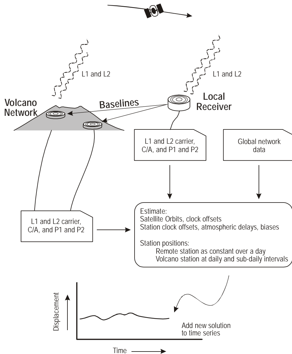
Figure 1-9. One possible design for a real-time, continuous, GPS volcano-monitoring system. Data collected at a volcano receiver are transmitted via modem to a central processing facility; this facility also collects data from other global and/or local receivers. Data from all receivers are “added” to the estimation of the baselines between the volcano monitoring stations and the local and/or global receivers. The processing facility monitors the GPS baseline results for strain accelerations. This information is used to adjust the frequency with which data are obtained from the volcano station for estimating relative motion. (from Webb and Bursik)
