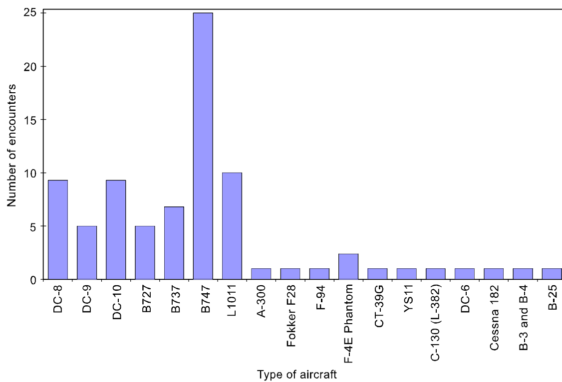
Figure 5. Plot showing the number of aircraft/volcanic ash encounters relative to the type of aircraft involved in the encounter
