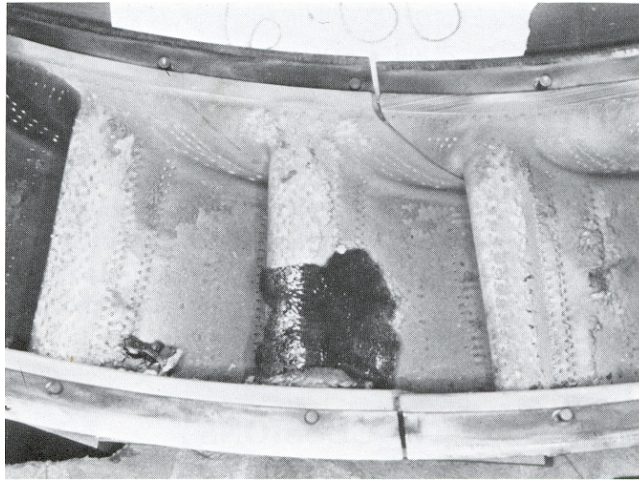
Figure 4-1 a). Dark, glassy deposits of remelted volcanic ash on leading edge of stage-1 high-pressure-turbine nozzle guide vane. (from Przedpelski and Casadevall)
