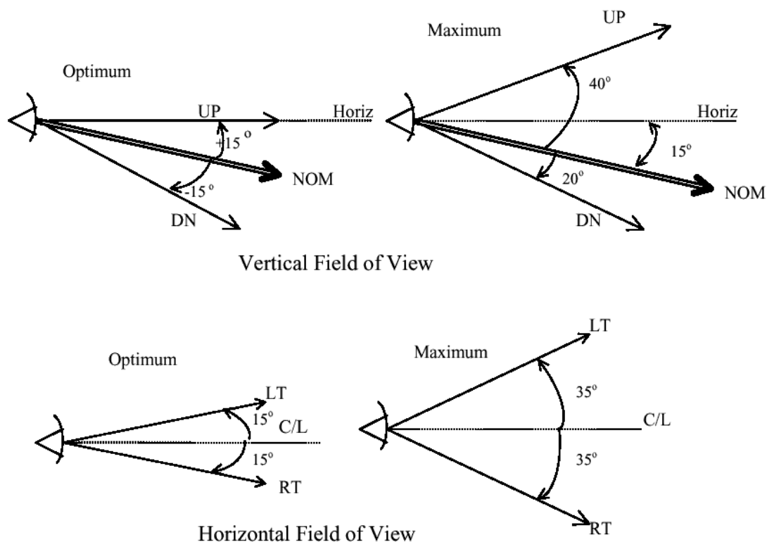
Figure C-2. Primary Field-of-View
