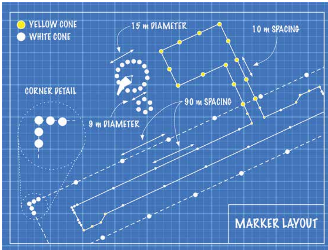
Figure 5: Marker Layout.
