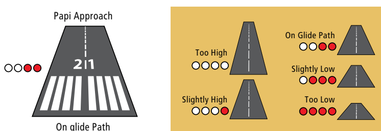
Figure 5: PAPI Lights – use of red and white provides glideslope indication
