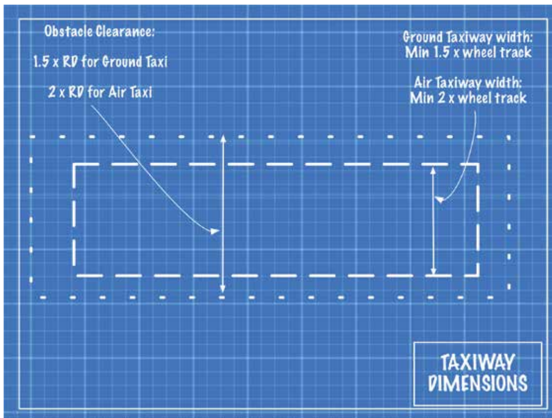
Figure 4: Helicopter taxiways
