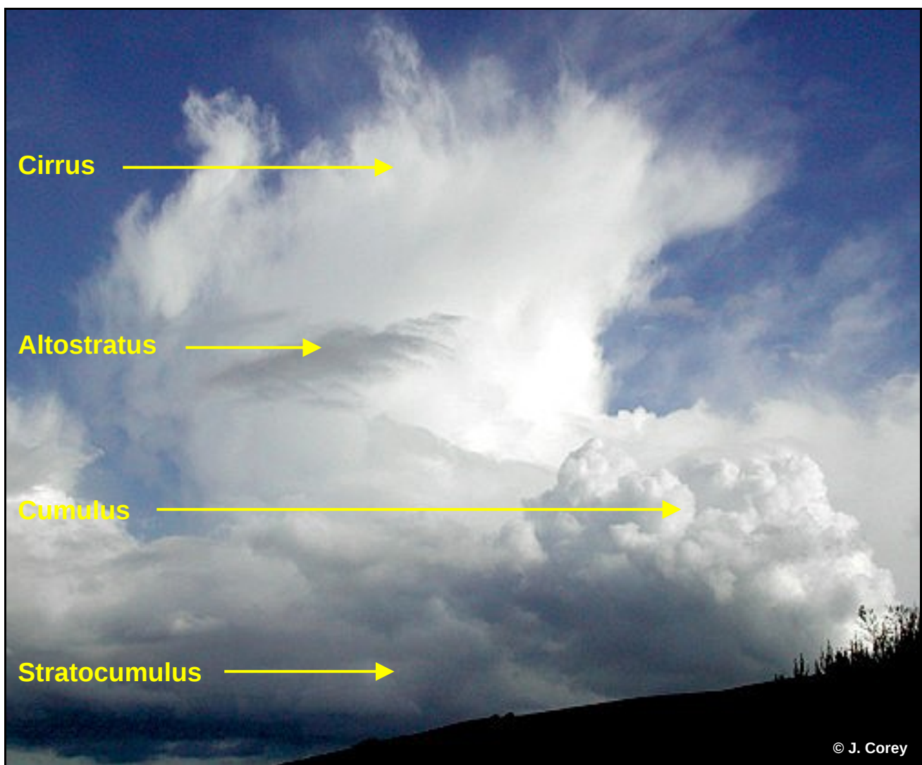
Figure 2. A cumulonimbus 'cloud factory'.
