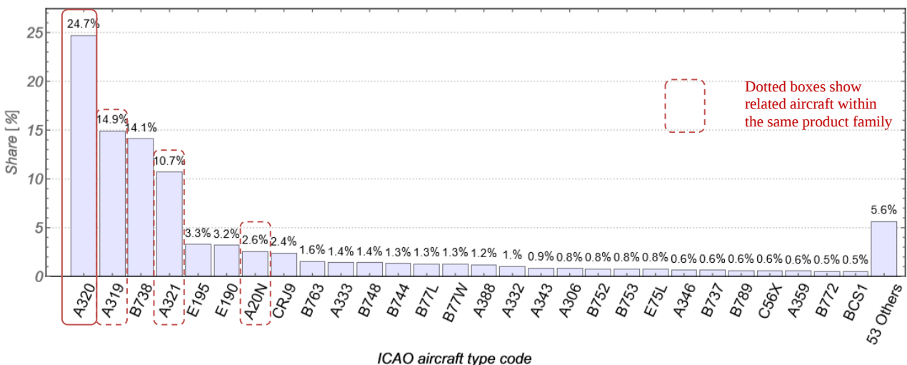
► Figure 3-3 ADS-B entries below FL120 for CS-25 jet airliners
