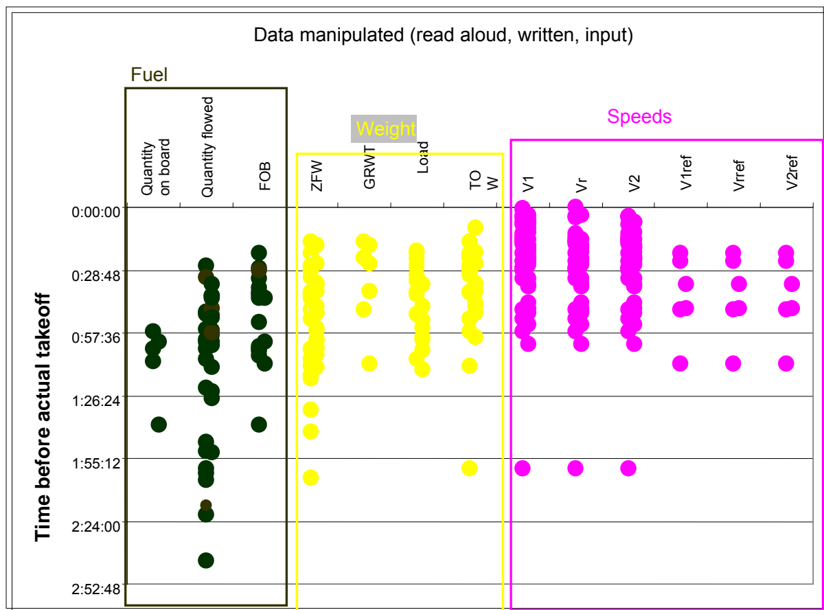
Figure 16: Data manipulated
