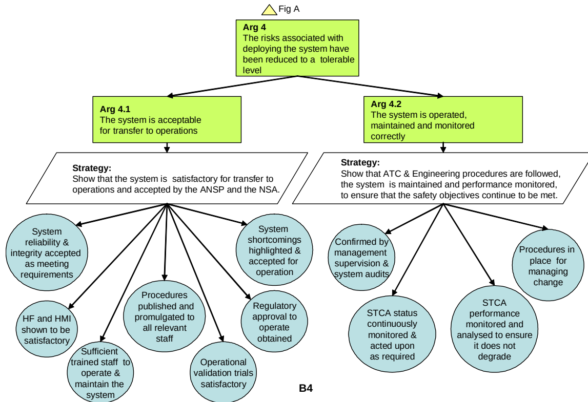
FIGURE B4 SYSTEM OPERATION & MAINTENANCE ASSURANCE
