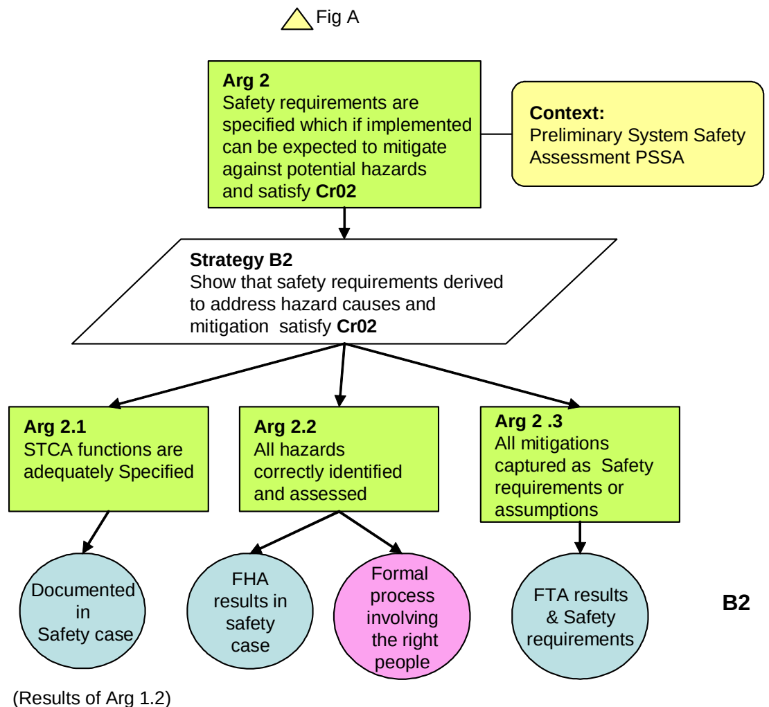
FIGURE B2 - SAFETY REQUIREMENTS ASSURANCE ARGUMENT
