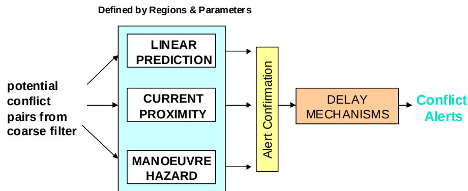
FIGURE 7.2 THE STCA FINE FILTERING STAGE
