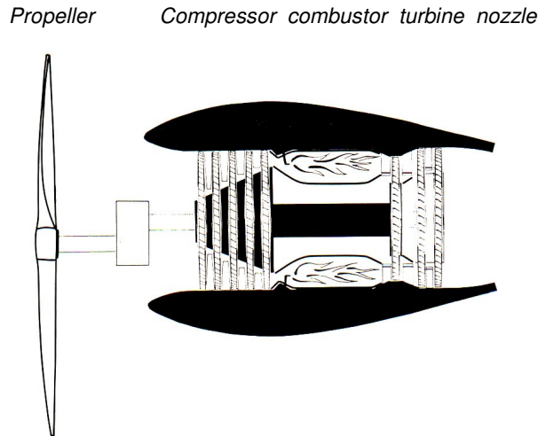
Figure 4 showing the basic layout of a turboprop propulsion system.
