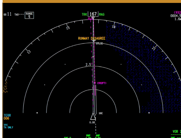
Figure 49. FMS runway disagree alert on the navigation display without airport map (© Boeing)
