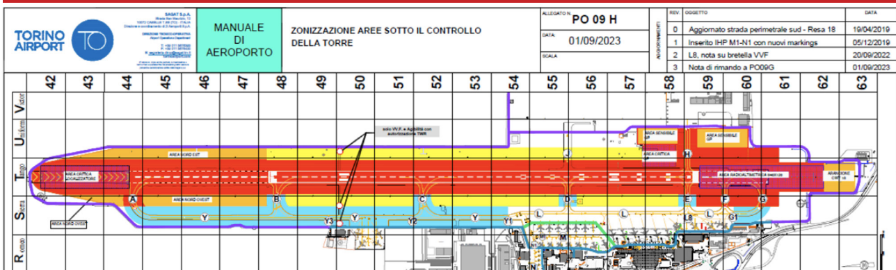
Figure 15. Torino Airport colour-based system
