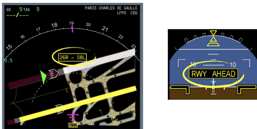
Figure 41. Airport moving map with aircraft location and visual advisory on the moving map, the primary flight display (PFD) and the head up display (HUD) when approaching a runway. Airbus A350 design shown.
